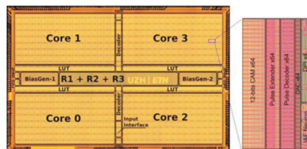
(b) DYNAPs [149]
