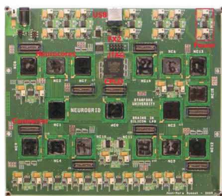
(a) Neurogrid [47]
